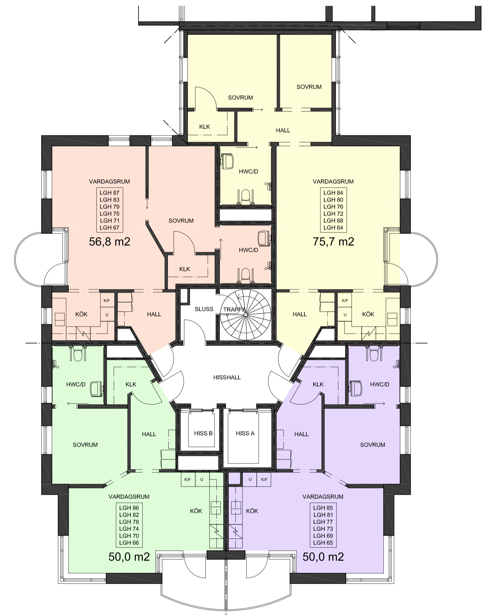
PLAN 3-8
